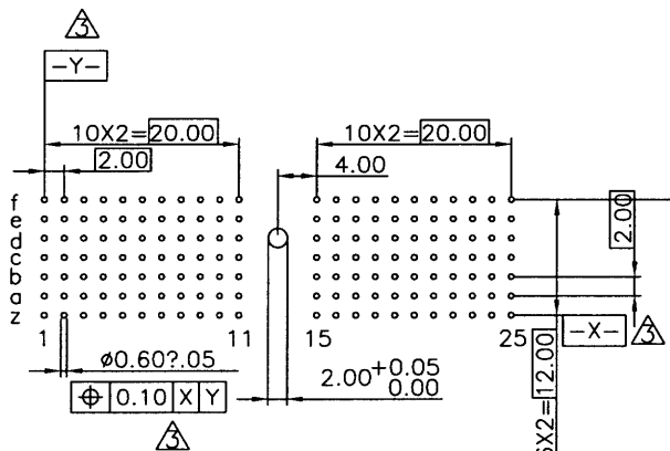
RECOMMENDED PCB-HOLE LAYOUT COMPONENT SIDE SHOWN TOLERANCES: ±0.05mm
