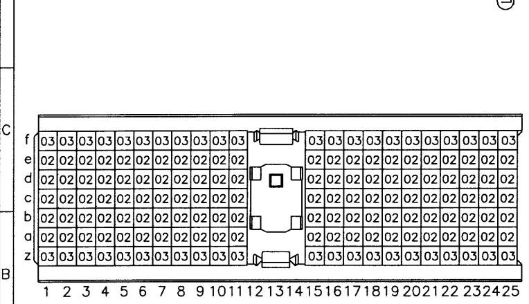
LOADING PATTERN MATING SIDE
