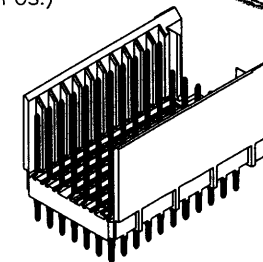
CONNECTOR ASSEMBLY EXEMPLARY LOADED
