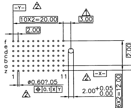
RECOMMENDED PCB-HOLE LAYOUT COMPONENT SIDE SHOWN TOLERANCES: ±0.05mm
